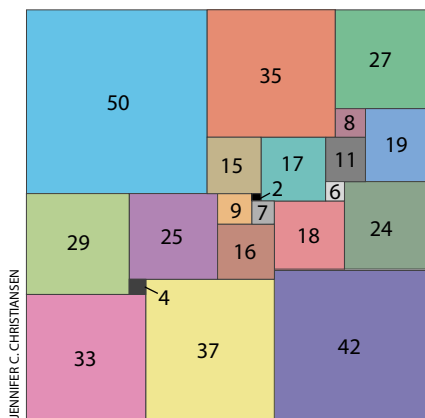
UNIQUE SQUARED SQUARE with the fewest tiles.
