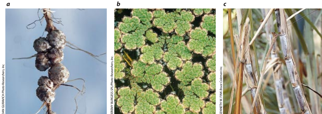
NITROGEN-FIXING BACTERIA , the microbes that convert atmospheric nitrogen into reactive compounds, live in root nodules of leguminous plants, such as soybeans (a). They can also be found in Azolla ferns (b) and inside sugarcane plants (c).
